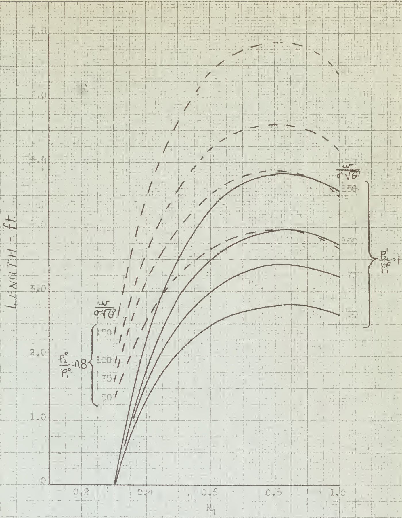
FIG. 17 - LENGTH OF CONICAL TUBES REQUIRED FOR VARIOUS MACH NUMBERS. EXIT MACH. NO. 0.5. DIVERGENCE ANGLE - 6^\circ .
